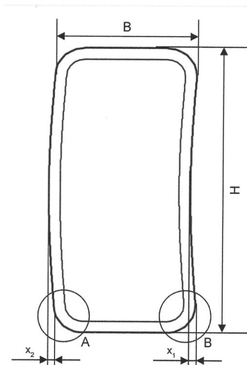
Figure 2 — Measurement of concavity/convexity of square or rectangular hollow sections
